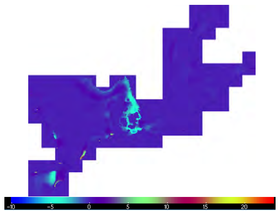
Figure 7. Difference in mean SSS in the North and Baltic Seas between coupled models and NEMO in January 1989
