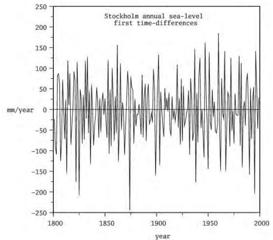
Figure 2. Time series of the first time differences, h(t+1)-h(t) , of the Stockholm annual sea-level.
