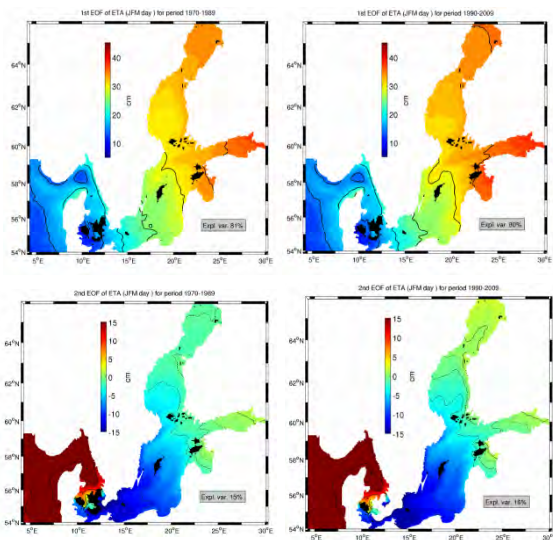
Figure 2. First and second EOF of winter (JFM) averaged daily SSEs BSIOM model output. Left panels for the period 1970-1989, right panels for the period 1990-2009.
