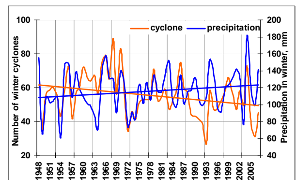
Figure 2. Dynamics of cyclones and precipitation in winter (December through February)
