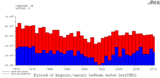
Figure 4. Extent of hypoxic (red) and anoxic (blue) bottom water in the Baltic Sea for the period 1970-2011.
