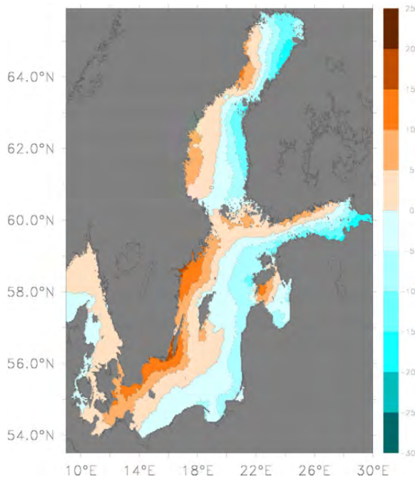
Figure 3: Ensemble mean summer net heat flux [ \text{W/m}^2 ] difference between the two climatological periods 2020 - 2049 and 1970 - 1999.
