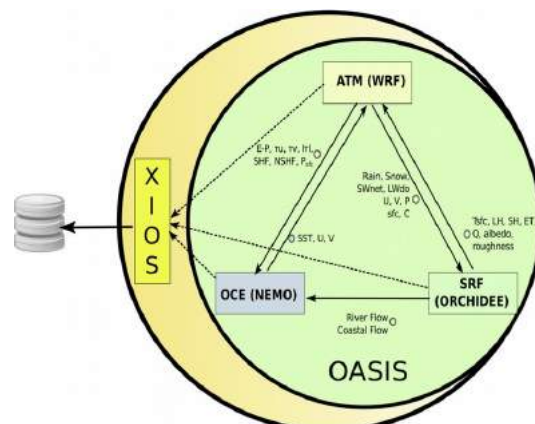
Figure 2. RegIPSL platform flow chart.
