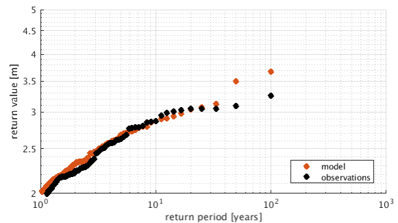
Figure 1. Return value plot of modeled (red) and observed (black) hourly sea level at Husum. Both refer to sea level above mean high water. For comparative reasons only the last 100 model years are shown here.
