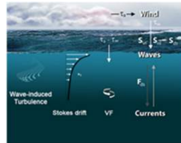
Figure 2. Wave induced processes into NEMO.
