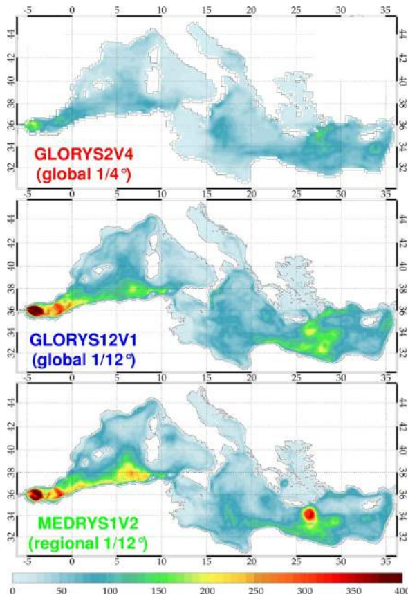
Figure 3. 40m-depth Eddy Kinetic Energy (EKE, in \text{cm}^2 \cdot \text{s}^{-2} ) in average over 1993-2012.
