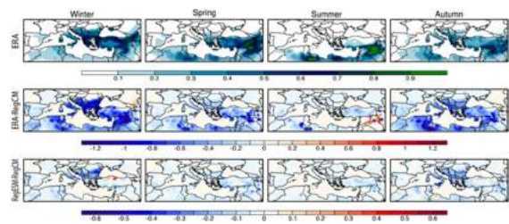
Figure 2. Seasonal precipitation sum of all regions over the Mediterranean Basin. First row shows Era-Interim, second row shows Era-Interim-RegCM4 and third row shows RegESM-RegCM.
