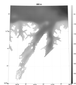
Figure 2. The grid of the Porsanger fjord ( \Delta x=800 m).
