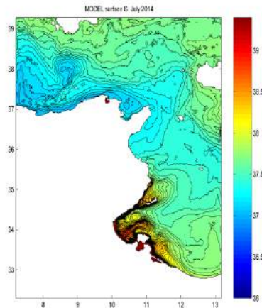
Figure 1. (a) Sea surface salinity from a collection of observations made during the summer season (June, July and August). (b) Sea salinity simulated by the INSTMCOTRHD model for the month of July. Depths less than 10 m are retained for observations and surface values are shown for the simulation. Units are PSU.
