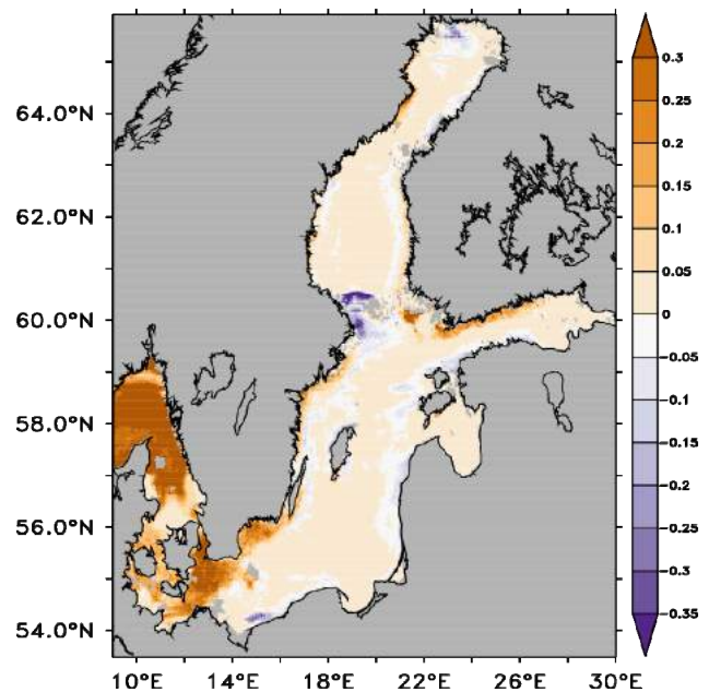
Figure 1. Changes in upwelling frequency [1] between the far future (2070 to 2099) and the recent past (1970 to 1999) for the RCP8.5 ensemble median. Values of 0.2 and above are significant and represent a change of 20%.
