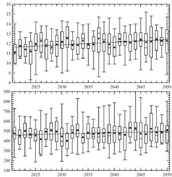
Figure 1. Annual mean temperature (°C; upper panel) and total precipitation (mm; lower panel) in Odessa estimated using the outcomes from the CORDEX Project
