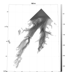
Figure 3. The grid of the Porsanger fjord ( \Delta x=160 m).
